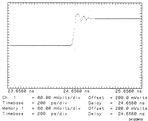
Figure 14-16. Reflected Edge Normalized to 16 ps Risetime Stimulus
