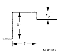
Figure C-5. Oscilloscope Display When E_r \neq 0
