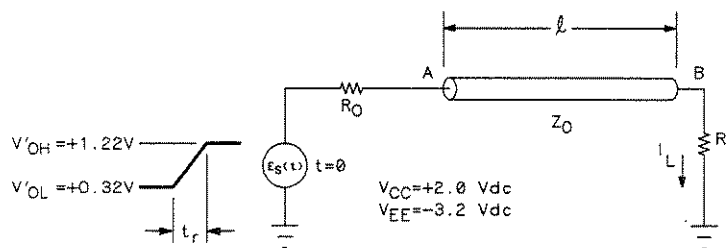
Figure E-3. Equivalent MECL Gate Output, Driving a Transmission Line
