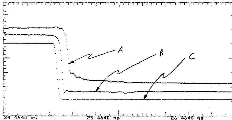
Figure C-27. Short Cables (B) and Normalization (C) can Reduce the Effects of Cable Loss Seen in (A)
