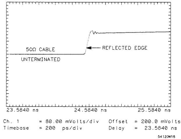
Figure 14-15. Reflected Edge
