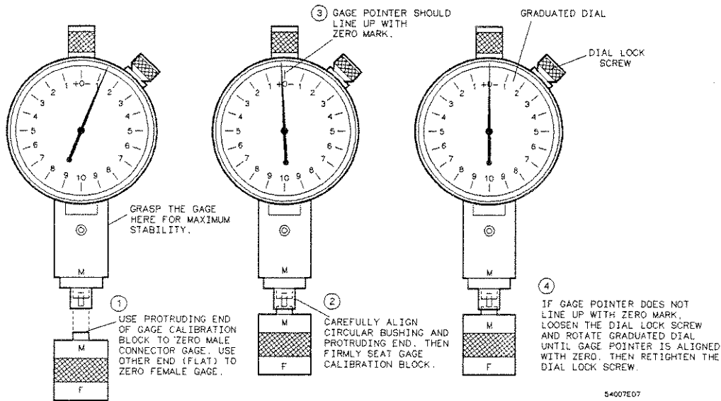
Figure B-7. Zeroing Precision 3.5 mm Connector Gauges
