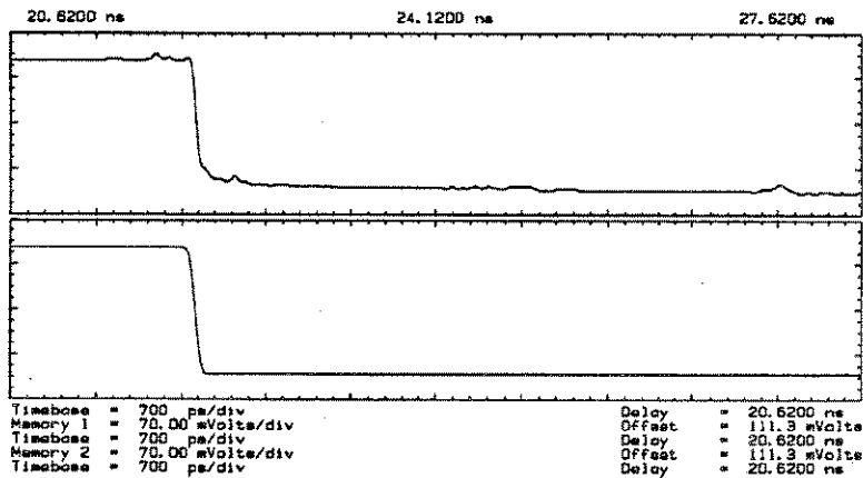
Figure D-1. The top waveform shows distortions caused by cables and connectors. The bottom waveform shows how normalization corrects for these distortions
