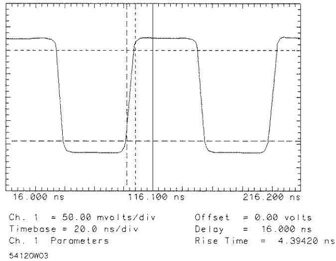
Figure 8-5. Risetime Measurement without Jitter (Averaged Mode)
