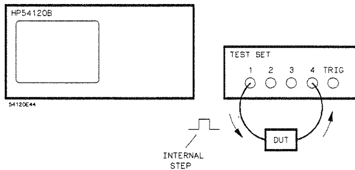
Figure 14-19. Transmission Measurement
