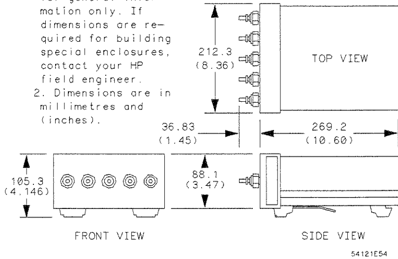
Figure 19-2. Four Channel Test Set dimensions
