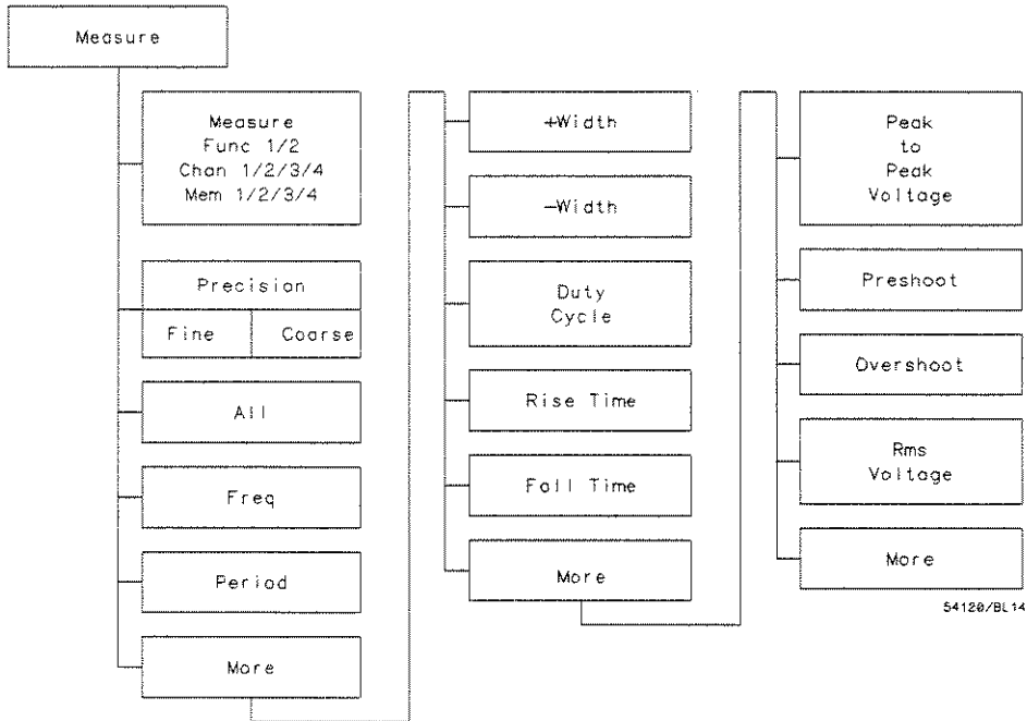
Figure 13-1. Measure Menu
