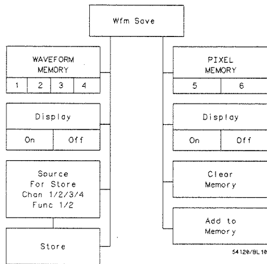
Figure 9-1. Waveform Menu
