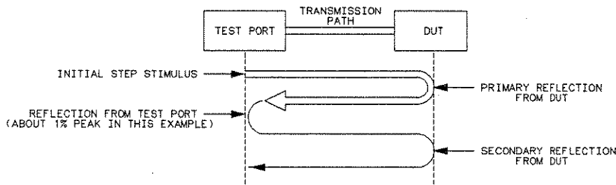
Figure D-11. By adding a section of airline between the test port and the DUT, you can more clearly distinguish primary and secondary reflections
