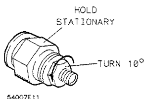
Figure B-11. Counter-Rotation Technique
