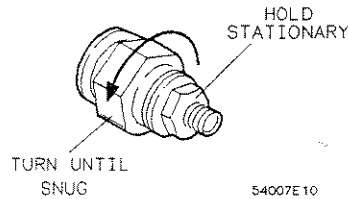
Figure B-10. Connecting 3.5 mm Devices
