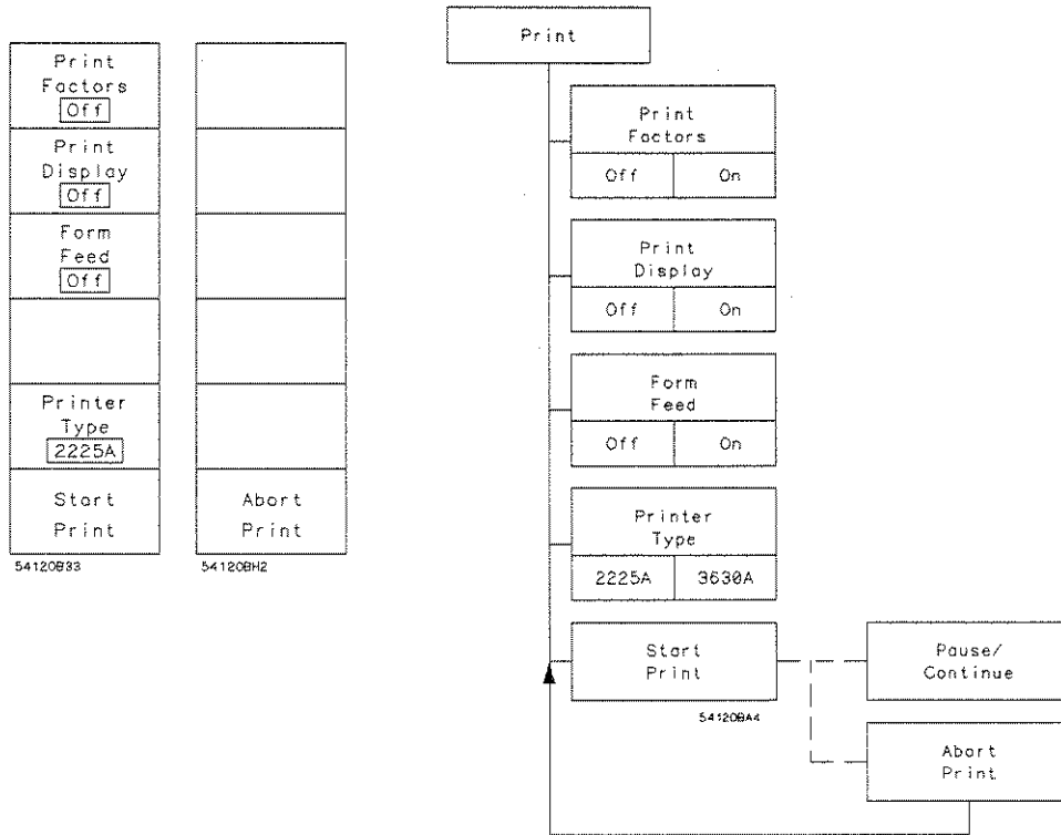
Figure 16-1. Print Menu
