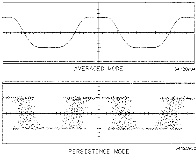
Figure 8-6. The Persistence and Averaged Display Modes with Time Jitter
