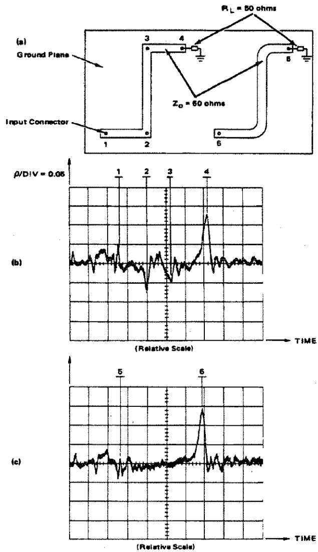
Figure E-17. Reflections Caused by Signal-Line Shape Variations
