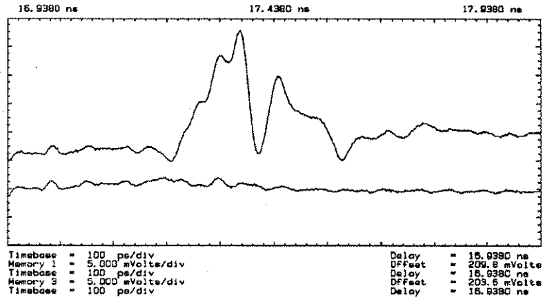
Figure D-9. Errors present in the TDR calibration waveform (bottom) are visible in the measured waveform (top)
