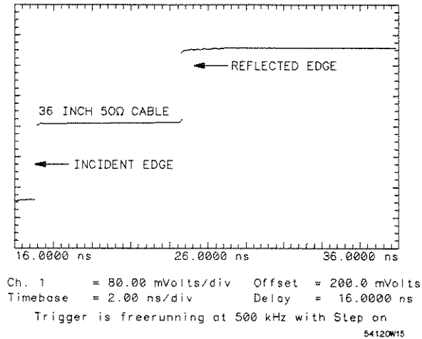
Figure 14-12. TDR Step
