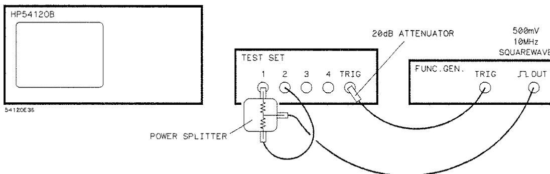
Figure 11-5. Equipment Configuration
