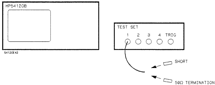
Figure 14-7. Reflect Cal
