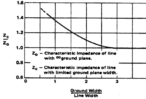
Figure E-12. Variation of Microstrip Impedance as a Function of Ground Width - Line Width
