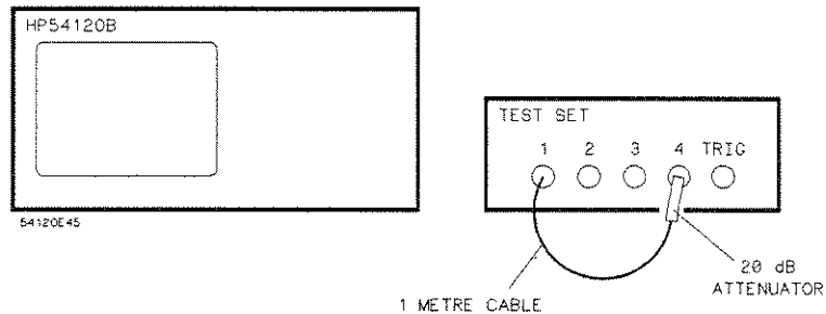
Figure 14-20. TDT Exercise Equipment Configuration
