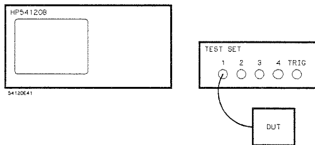
Figure 14-4. TDR Measurement
