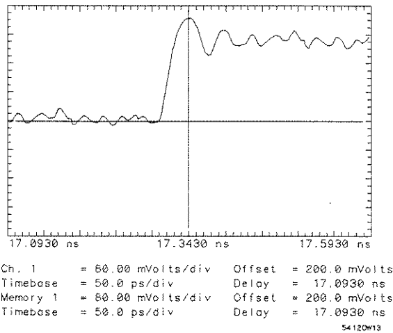
Figure 14-8. Instability Caused by Low Number of Averages When 10 ps Normalized Risettime Is Used
