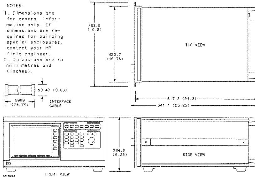
Figure 19-1. 54120B Dimensions
