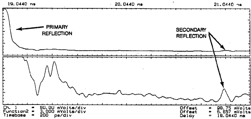
Figure D-10. The lower waveform is a copy of the upper waveform with the voltage scale greatly expanded about the baseline to show more clearly the shape of the secondary reflection
