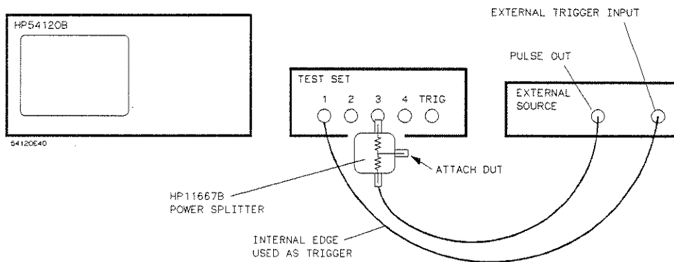
Figure 14-5. TDR Using an External Pulse Source
