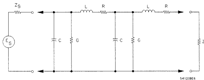
Figure C-2. The Classical Model for a Transmission Line.
