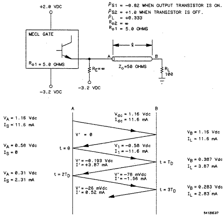
Figure E-5. Lattice Diagram for Negative-Going Voltage Transition
