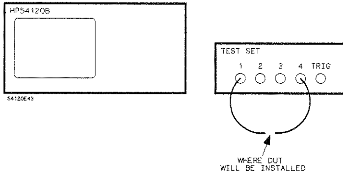
Figure 14-9. Transmission Cal
