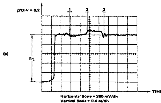
Figure E-15. Hybrid Divider with Crosstalk Problem
