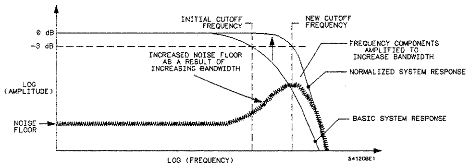
Figure D-15. Normalized system frequency response (system bandwidth increased)
