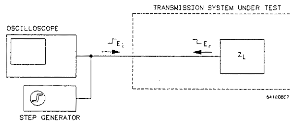
Figure C-3. A Time Domain Reflectometer
