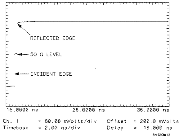
Figure 14-3. Internal Step
