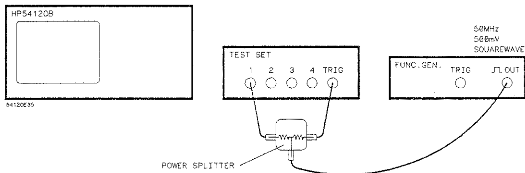
Figure 10-2. Equipment Configuration
