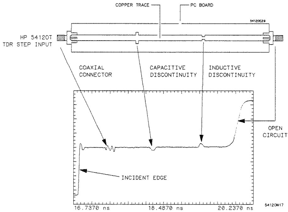
Figure 14-14. TDR Step with a Strip Line
