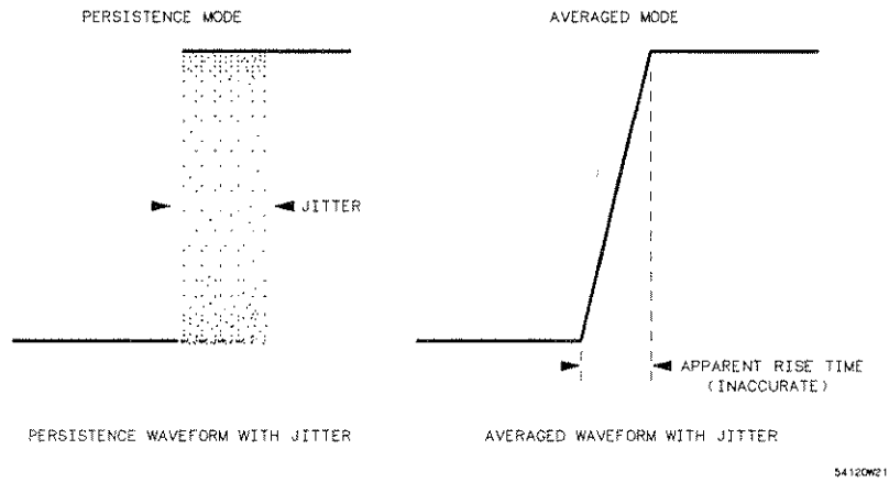
Figure 8-7. Time Jitter with Persistence display mode
