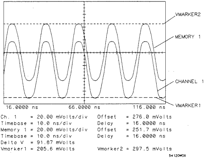
Figure 10-5. Source-to-Source Voltage Measurement
