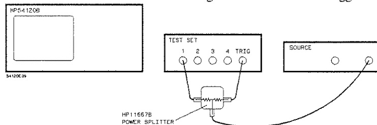
Figure 3 - 1. Acquiring a Waveform
