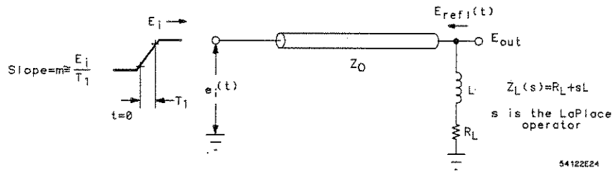
Figure E-9. Circuit for Determining the Maximum Reflected Voltage Due to the Inductance of the Resistor Leads
