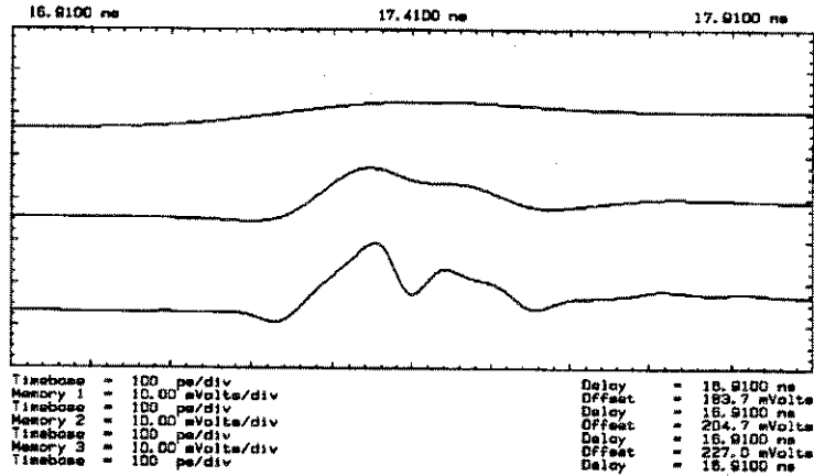
Figure D-2. Variable edge speed helps determine the amount of reflection in actual applications. The top waveform (tested to 350 ps) shows less reflection than the middle waveform (tested to 100 ps) or the bottom waveform (tested to 50 ps)
