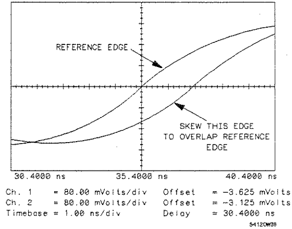
Figure 18-3. Reference Edge and Channel with Time Differential
