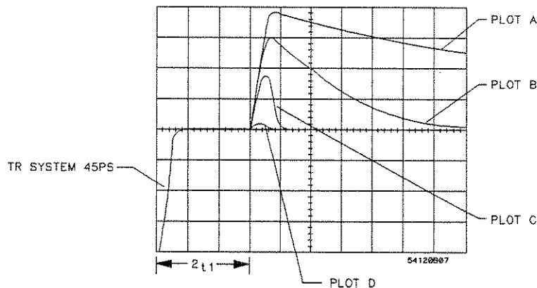
Figure C-26. System Risetime Affects the TDR Results
