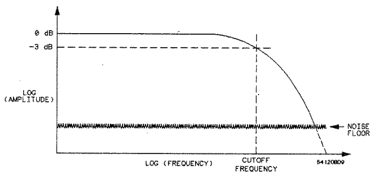
Figure D-13. Basic system frequency response
