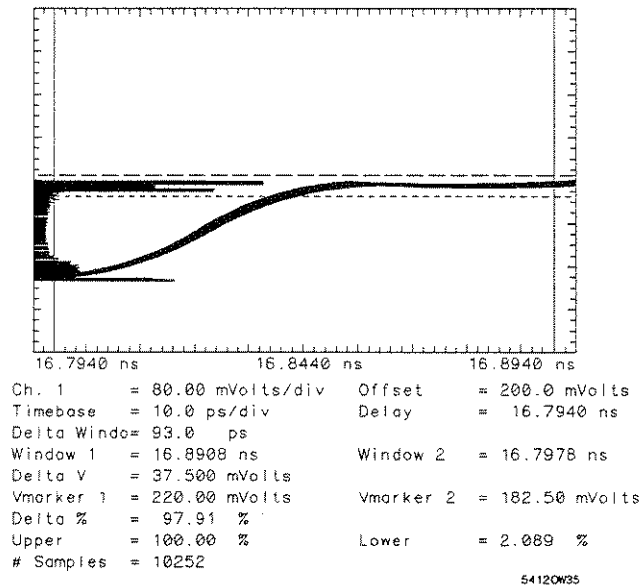
Figure 15-7. Evaluating the Distribution on a Multimodal Signal
