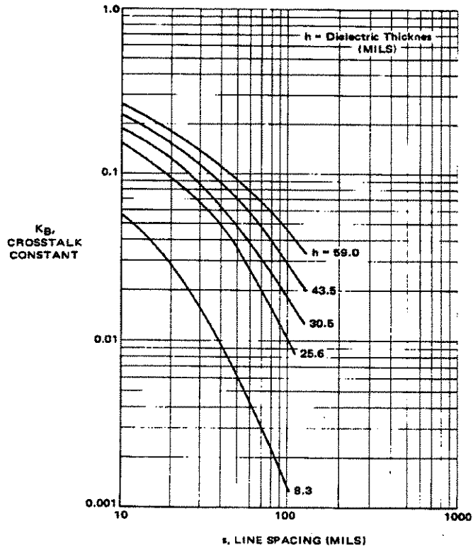
Figure E-16. Backward Crosstalk Coefficient for Microstrip Lines on Glass Epoxy Boards (G-10 Material)
