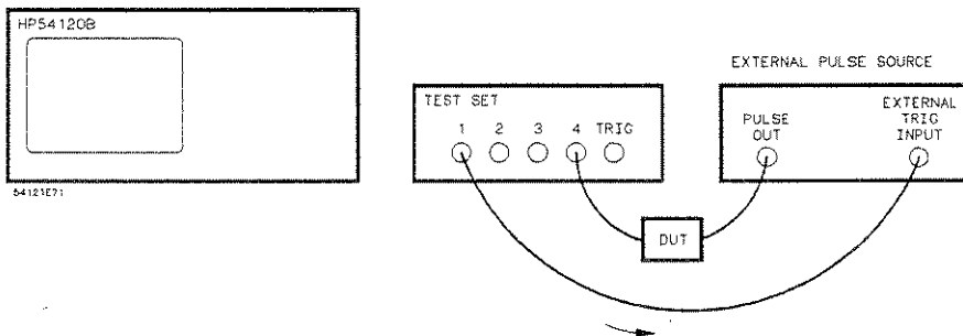
Figure 14-23. TDT Transmission Test Using External Pulse Source
