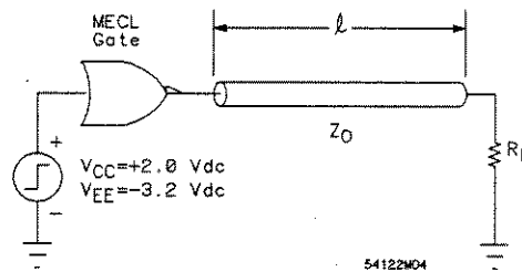
Figure E-2. MECL Gate Driving a Transmission Line
