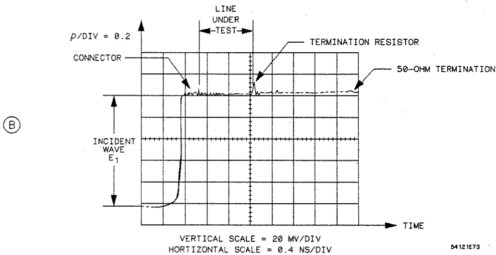
Figure E-8B and C. TDR Determination of Line Characteristic Impedance (Continued)
