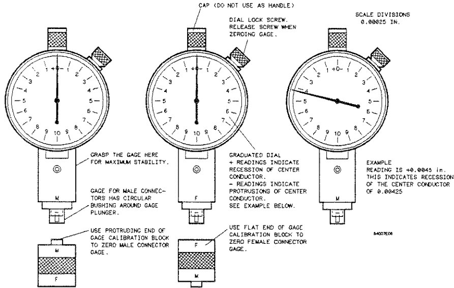
Figure B-6. Precision 3.5 mm Connector Gauges
