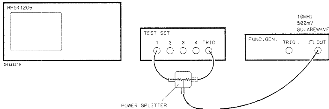
Figure 8-2. Equipment Configuration.
