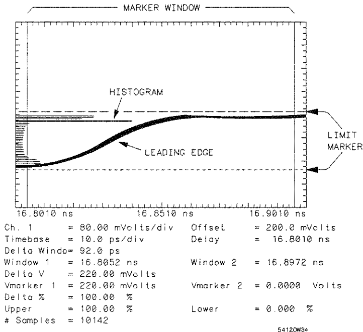
Figure 15-6. Voltage Histogram
