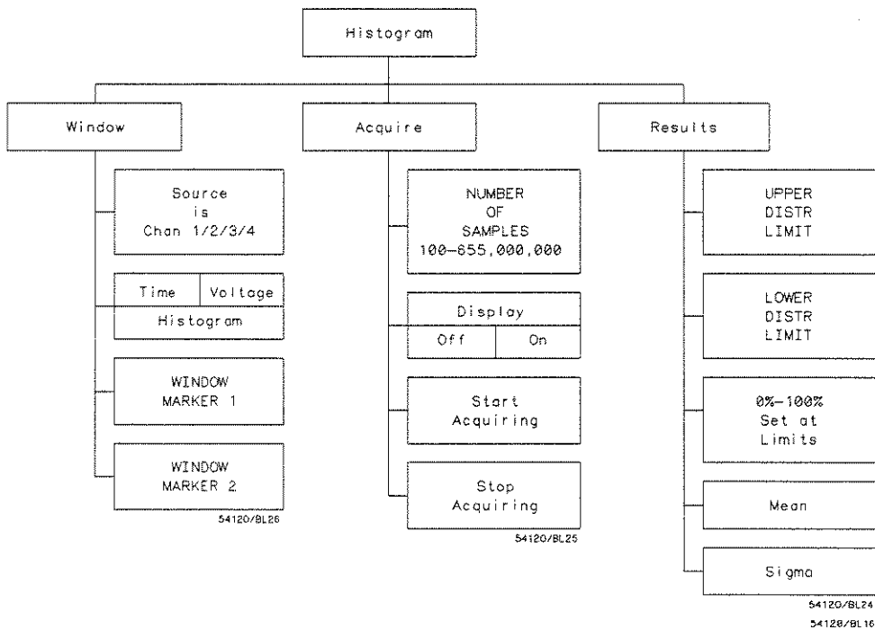
Figure 15-1. Histogram Menu Schematic
