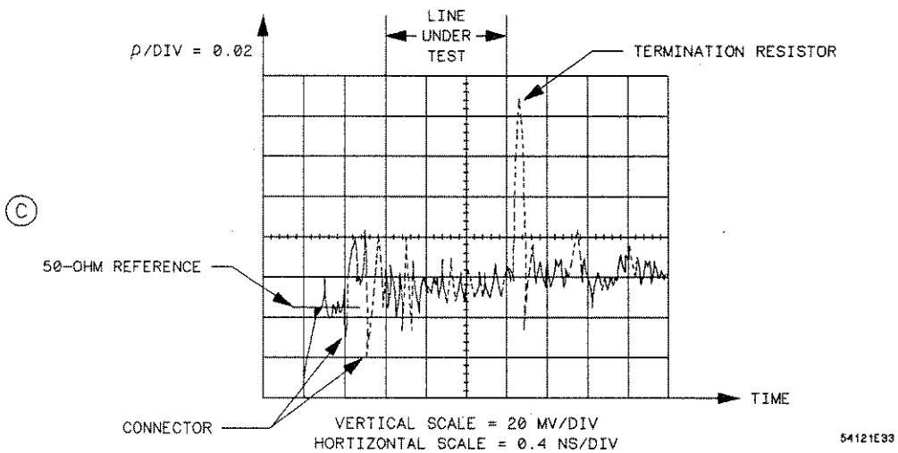
Figure E-8C. TDR Determination of Line Characteristic Impedance (Continued)
