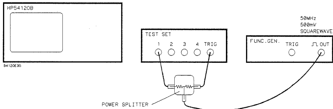
Figure 11-3. Equipment Configuration
