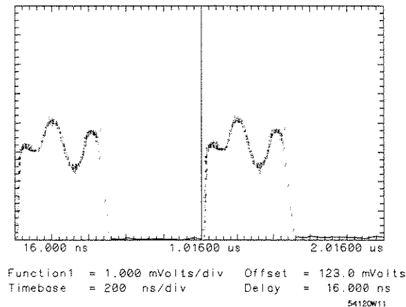
Figure 12-4. Using the Only Operator
