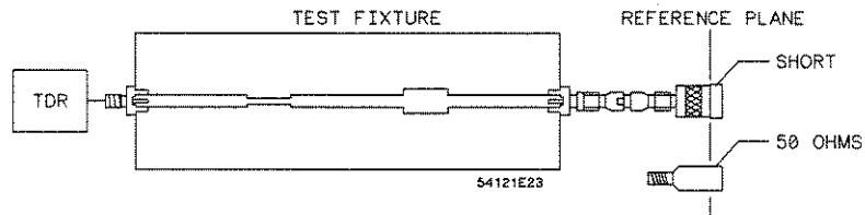
Figure D-5. A normalization calibration uses first a short, then a 50 \Omega termination to define a reference plane and generate a digital filter
