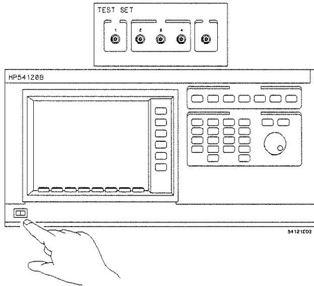
Figure 2-2. HP 54121T Front Panels
