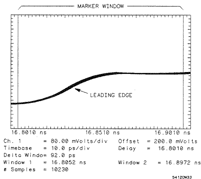
Figure 15-5. Leading Edge
