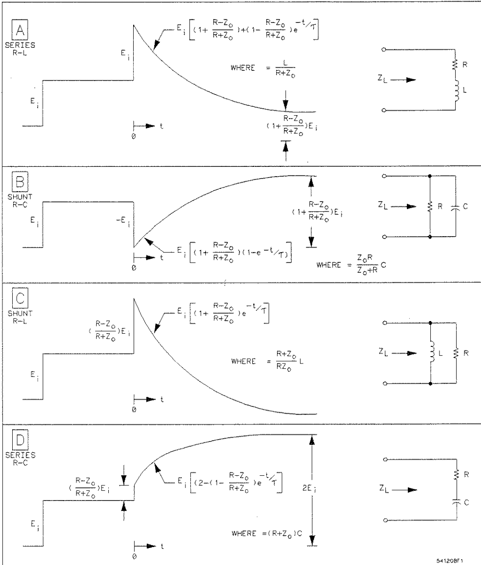
Figure C-7. Oscilloscope Displays for Complex Z_L
