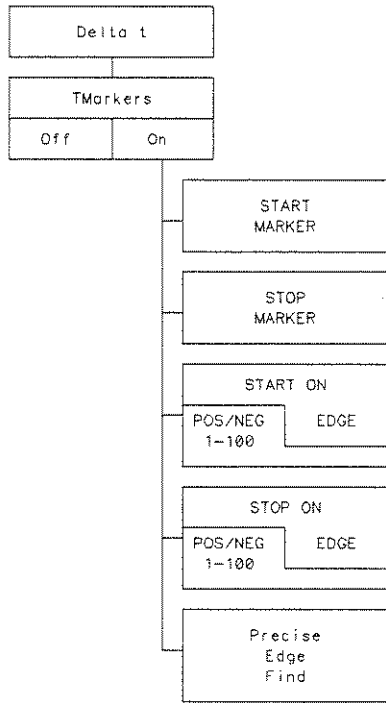
Figure 11-1. Delta t Menu
