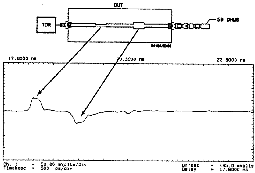
Figure D-7. The unnormalized response of the DUT, measured without the test fixture
