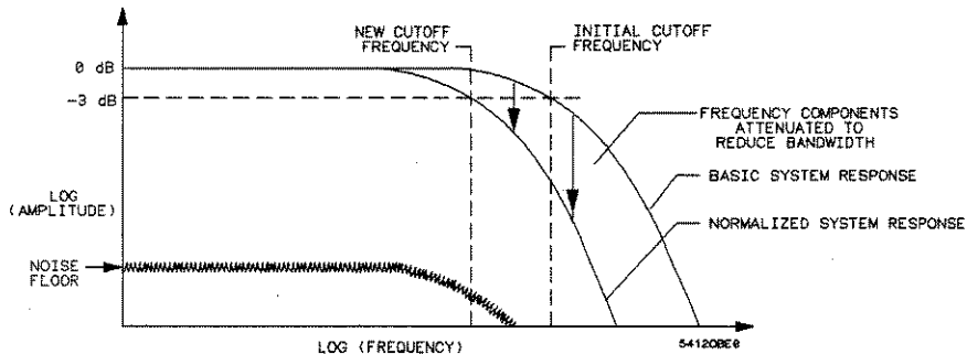
Figure D-14. Normalized system frequency response (system bandwidth reduced)
