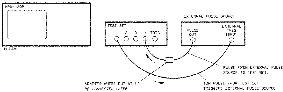
Figure 14-22. Thru Cal Using External Pulse Source
