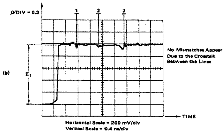
Figure E-14. Hybrid Divider
