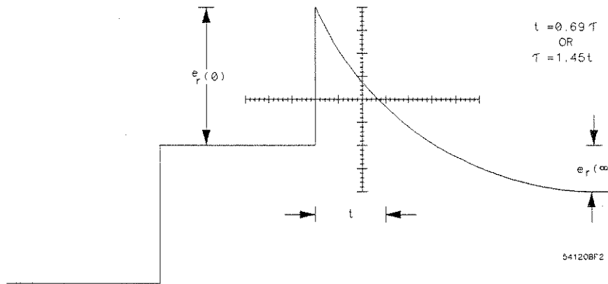
Figure C-8. Determining the Time Constant of a Reflected Wave Returning from a Complex Z_L
