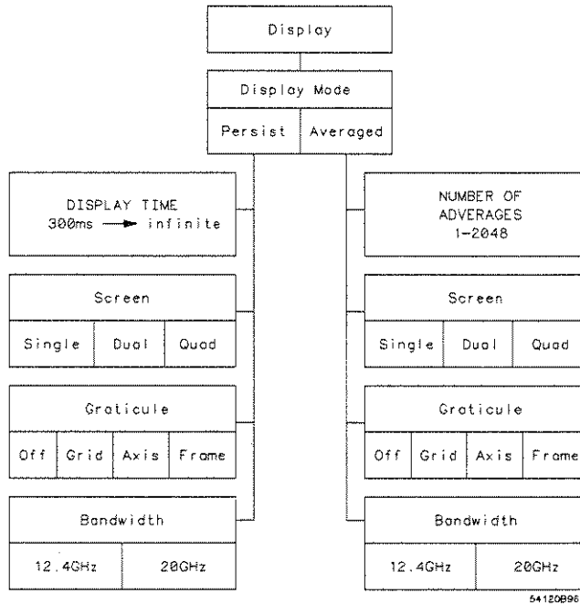
Figure 8-1. Display Menu
