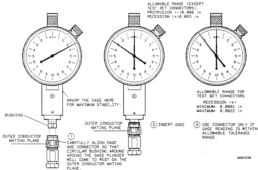
Figure B-8. Measuring Precision 3.5 mm Male Connectors
