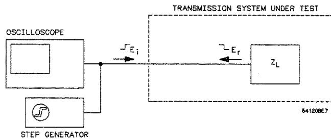
Figure E-7. Time Domain Reflectometer
