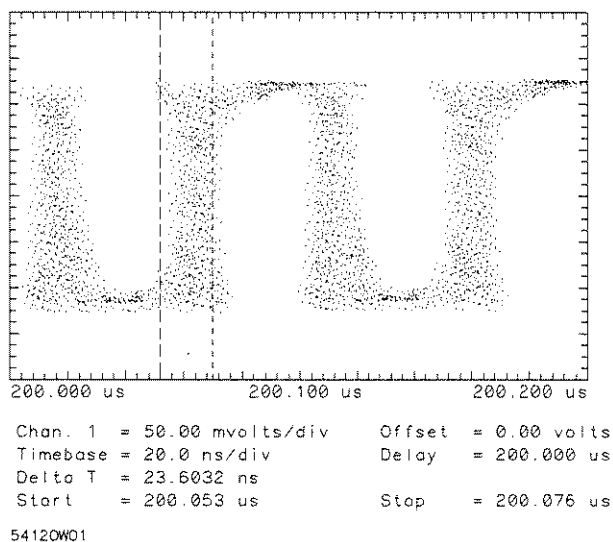
Figure 8-3. Jitter in Persistence Mode
