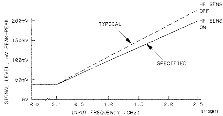
Figure 7-1. Trigger Sensitivity
