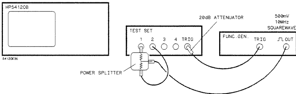
Figure 12-2. Equipment Configuration
