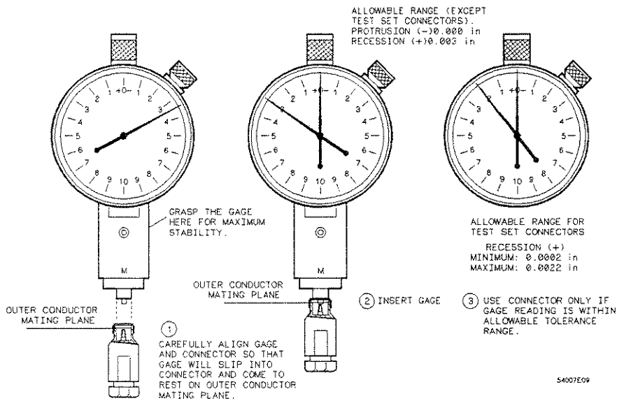
Figure B-9. Measuring Precision 3.5 mm Female Connectors
