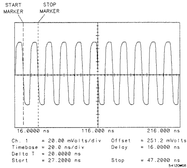
Figure 11-4. Pulse Period
