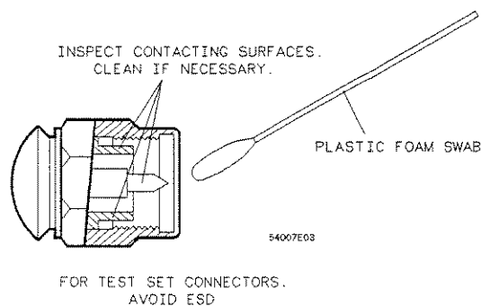
Figure B-3: Visual Inspection of 3.5 mm Connectors
