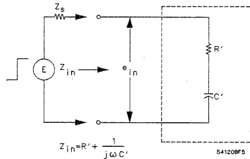
Figure C-12. A Simple Model Valid at t = 0^+ for a line with series losses
