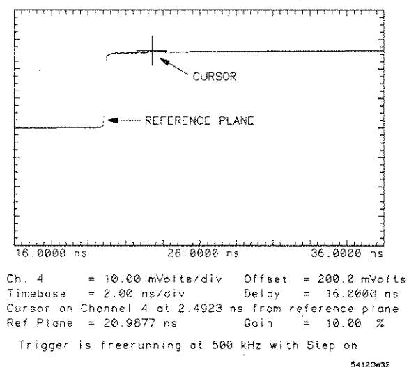
Figure 14-21. Cursor on a Transmission Waveform
