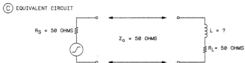
Figure E-10. Effects Due to Termination Resistor Leads
