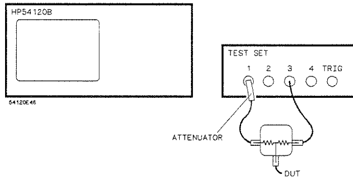
Figure 14-6. TDR with Attenuated Internal Step
