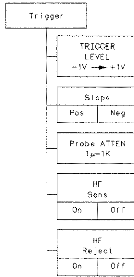
Figure 7-1. Trigger Menu
