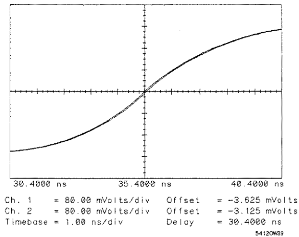
Figure 18-4. Reference Edge and Channel Overlapped
