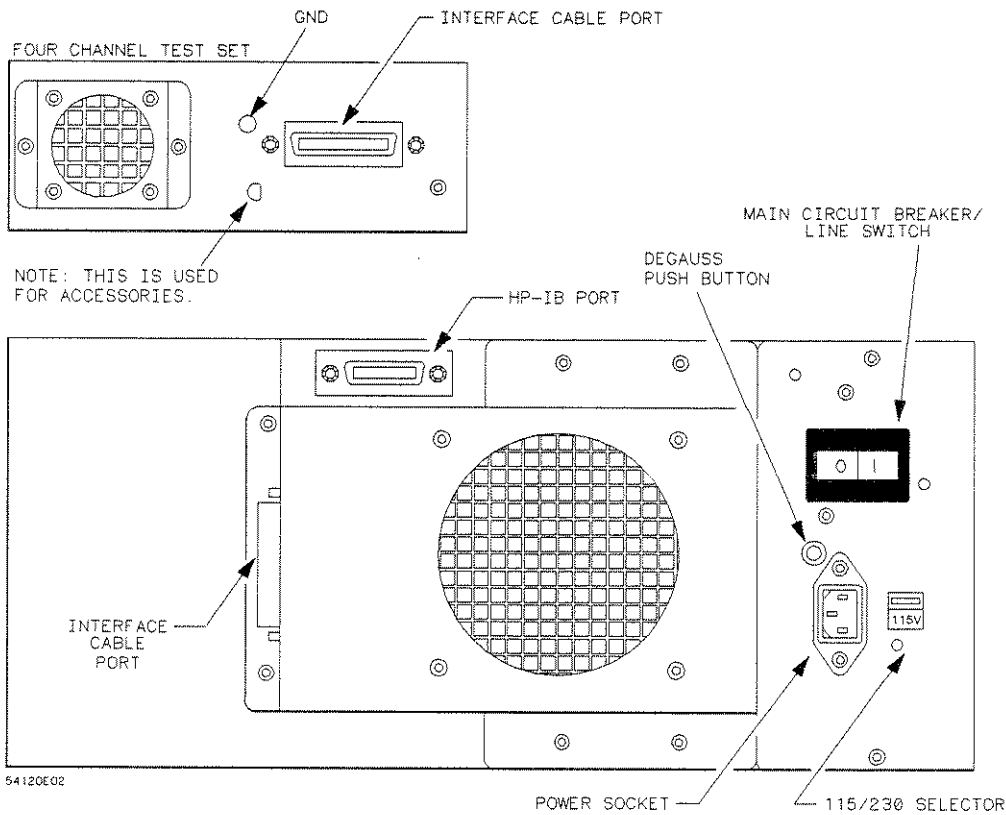
Figure 2-1. Power Module on Rear Panel
