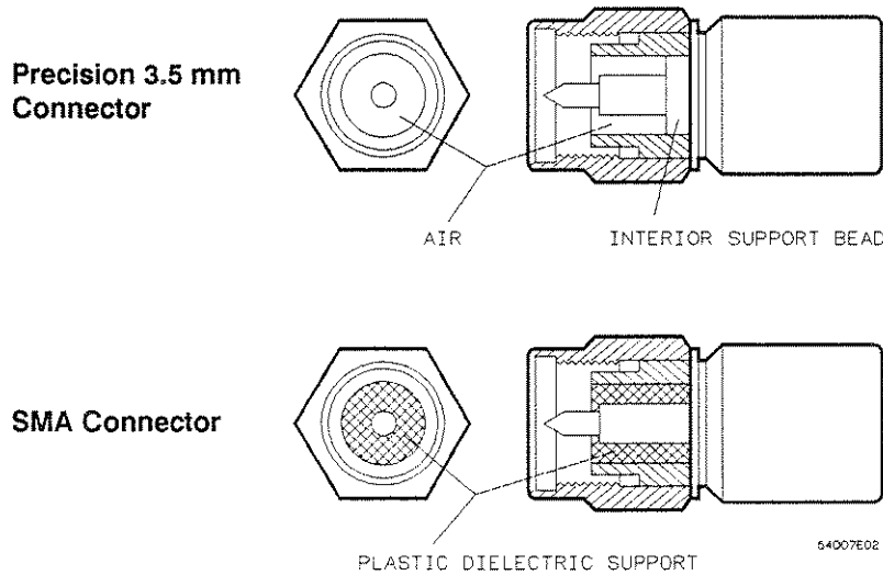
Figure B-1. SMA and Precision 3.5 mm Connectors
