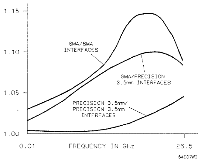
Figure B-2. Typical SWR of SMA and 3.5 mm Connectors
