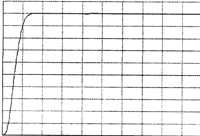
Figure C-31. Extra Capacitance can Compensate for the Wirebond's Inductance, Reducing the Reflection
