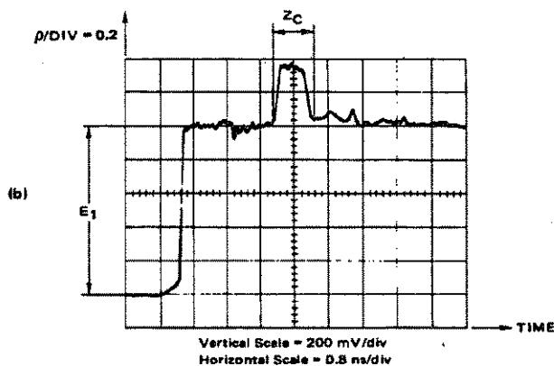
Figure E-13. Effects of Ground Plane Discontinuity
